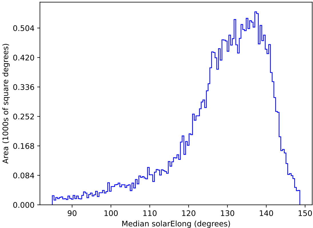
roll_pause_mjdp270_v3.4_10yrs All sky i band: Median solarElong
