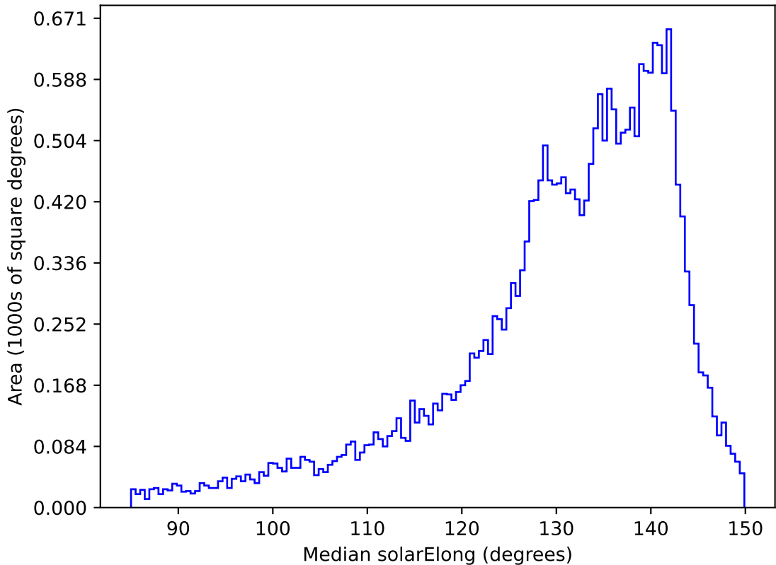
roll_pause_mjdp270_v3.4_10yrs All sky all bands: Median solarElong
