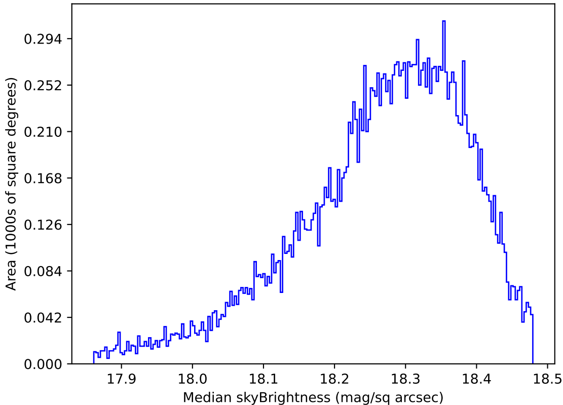
roll_pause_mjdp270_v3.4_10yrs Yr 1 y band: Median skyBrightness
