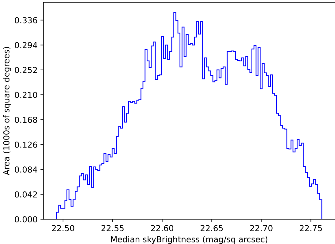
roll_pause_mjdp270_v3.4_10yrs Yr 1 u band: Median skyBrightness
