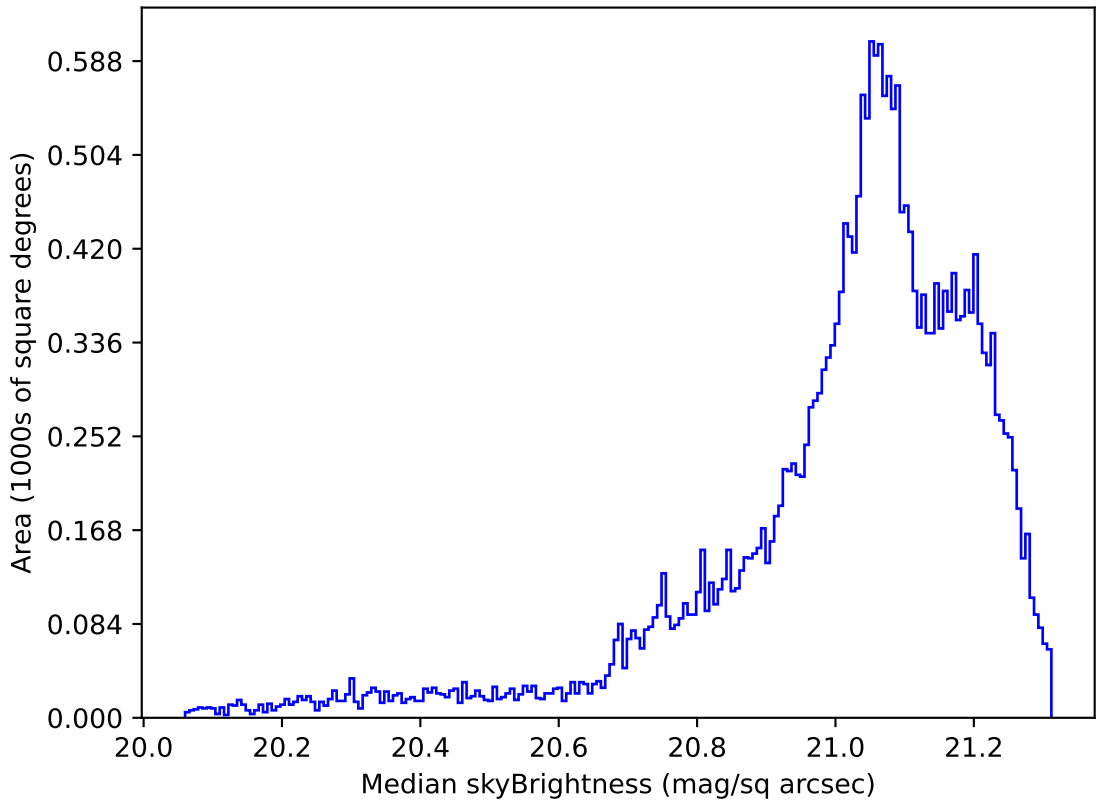
roll_pause_mjdp270_v3.4_10yrs Yr 1 r band: Median skyBrightness
