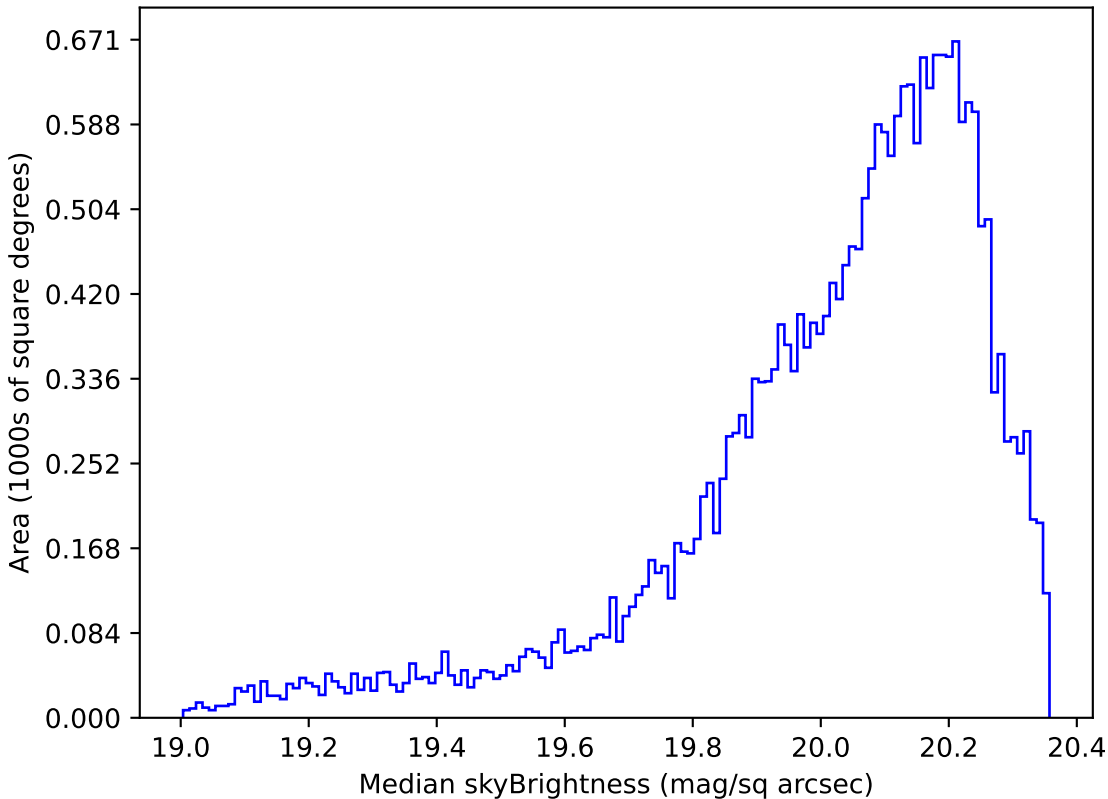
roll_pause_mjdp270_v3.4_10yrs Yr 1 i band: Median skyBrightness
