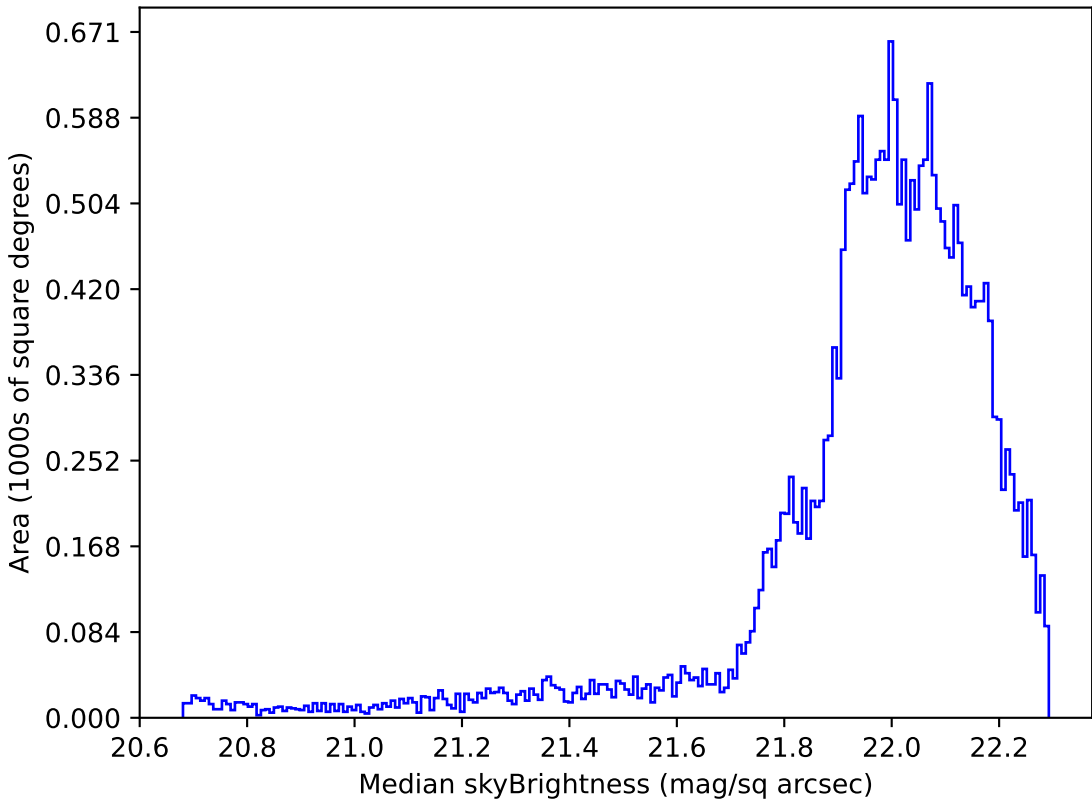
roll_pause_mjdp270_v3.4_10yrs Yr 1 g band: Median skyBrightness
