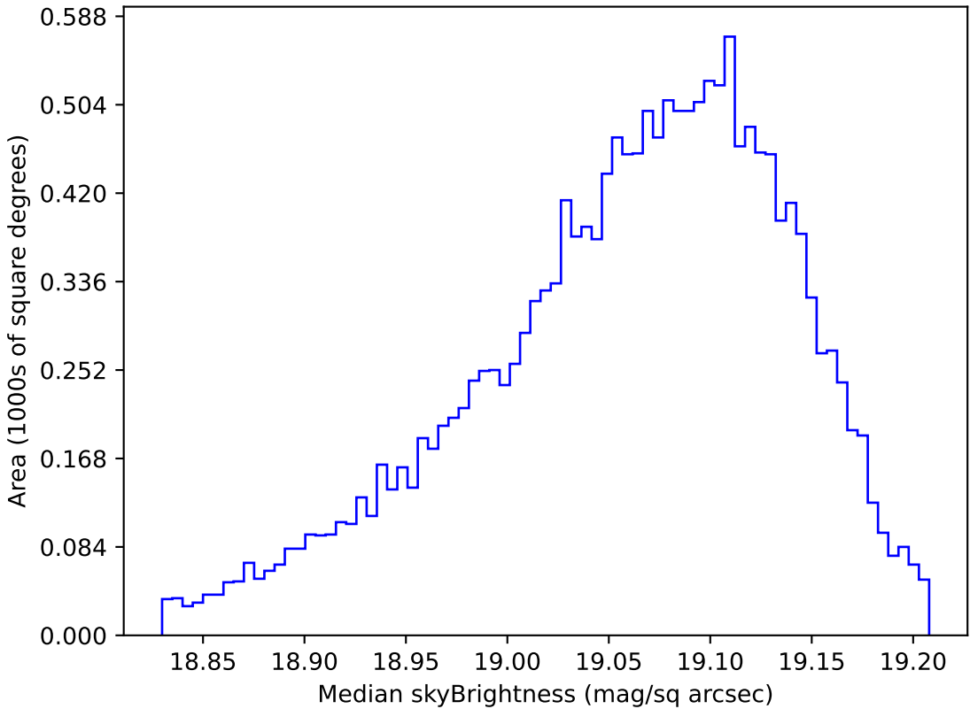
roll_pause_mjdp270_v3.4_10yrs WFD z band: Median skyBrightness
