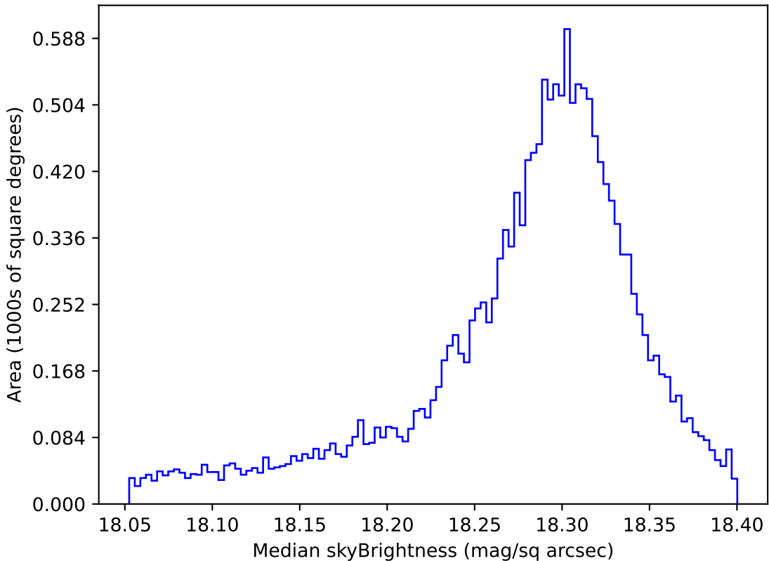
roll_pause_mjdp270_v3.4_10yrs WFD y band: Median skyBrightness
