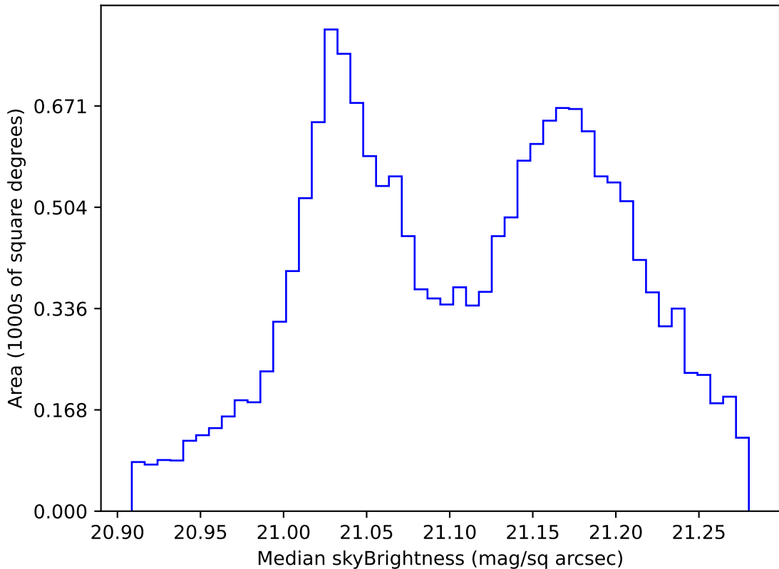
roll_pause_mjdp270_v3.4_10yrs WFD r band: Median skyBrightness
