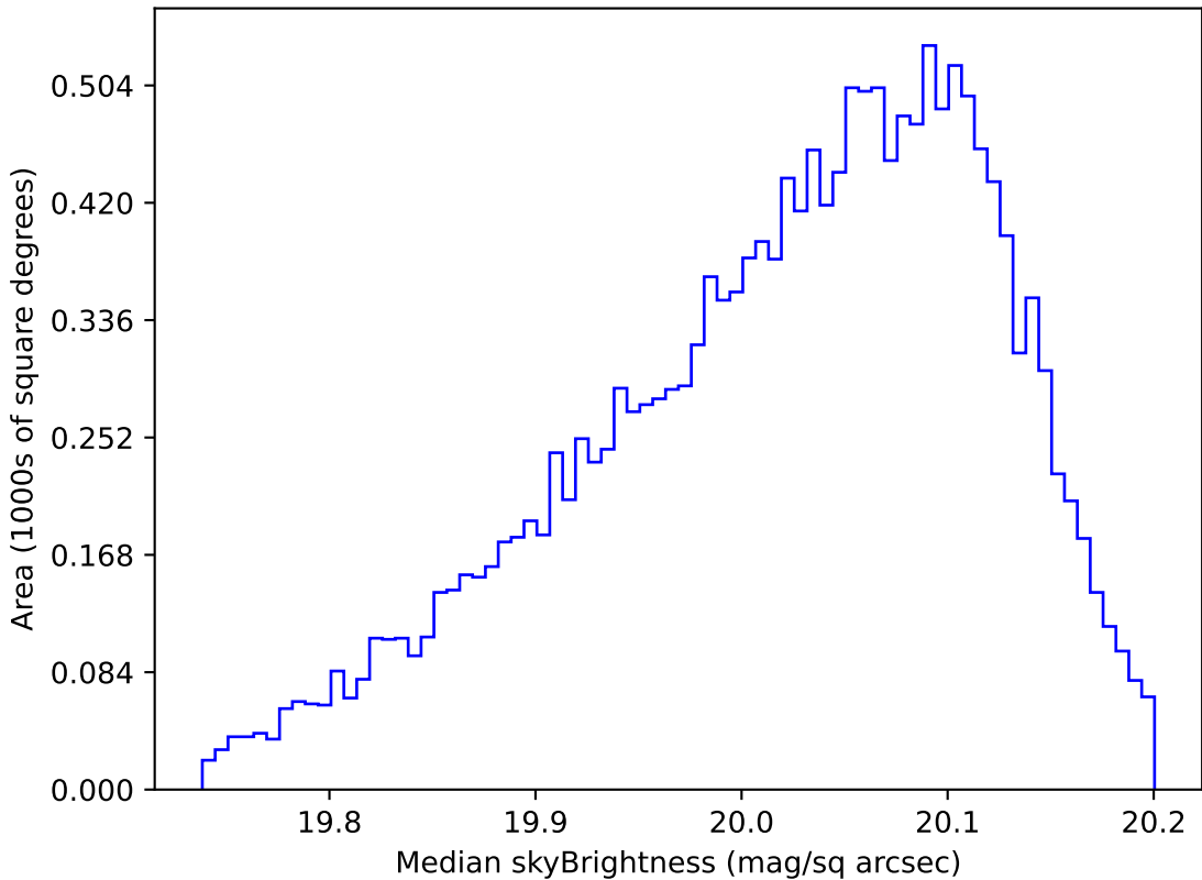
roll_pause_mjdp270_v3.4_10yrs WFD i band: Median skyBrightness
