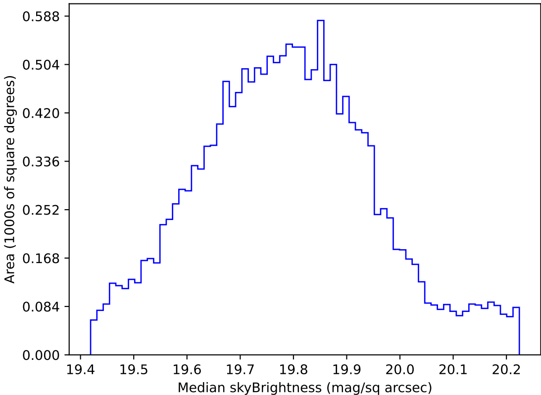
roll_pause_mjdp270_v3.4_10yrs WFD all bands: Median skyBrightness
