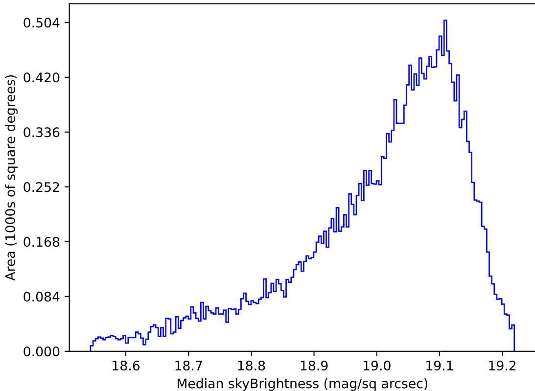
roll_pause_mjdp270_v3.4_10yrs All sky z band: Median skyBrightness
