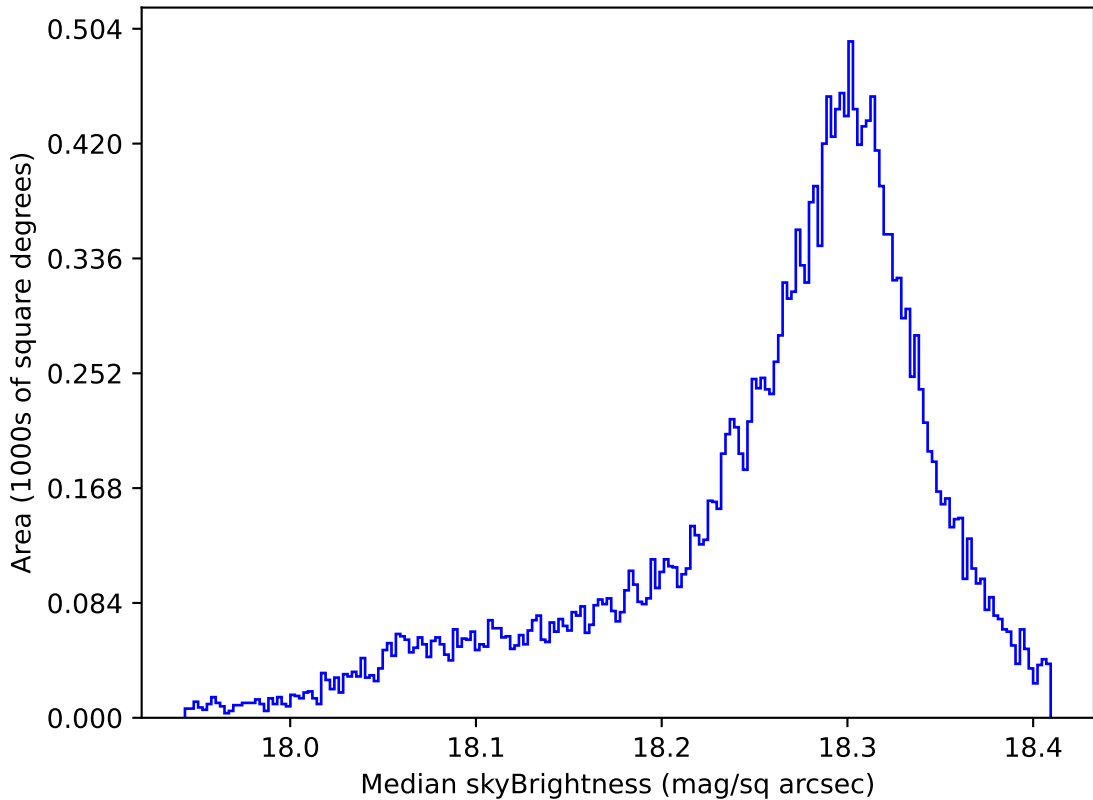
roll_pause_mjdp270_v3.4_10yrs All sky y band: Median skyBrightness
