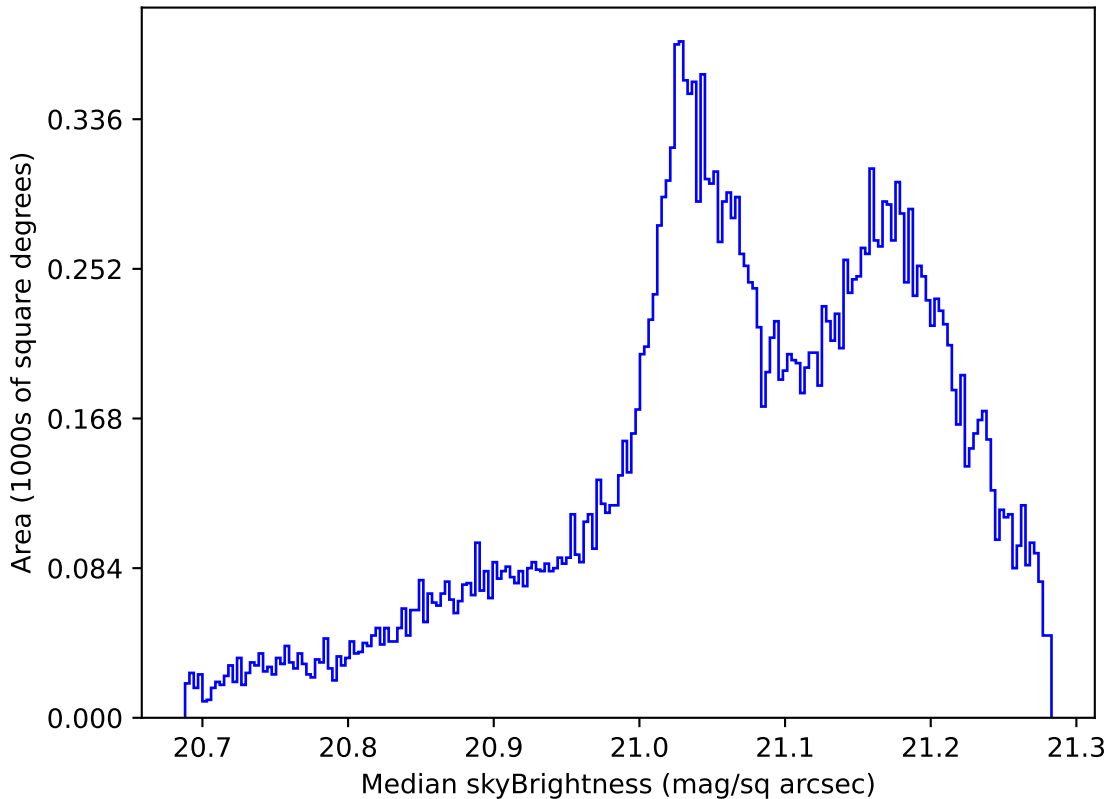
roll_pause_mjdp270_v3.4_10yrs All sky r band: Median skyBrightness
