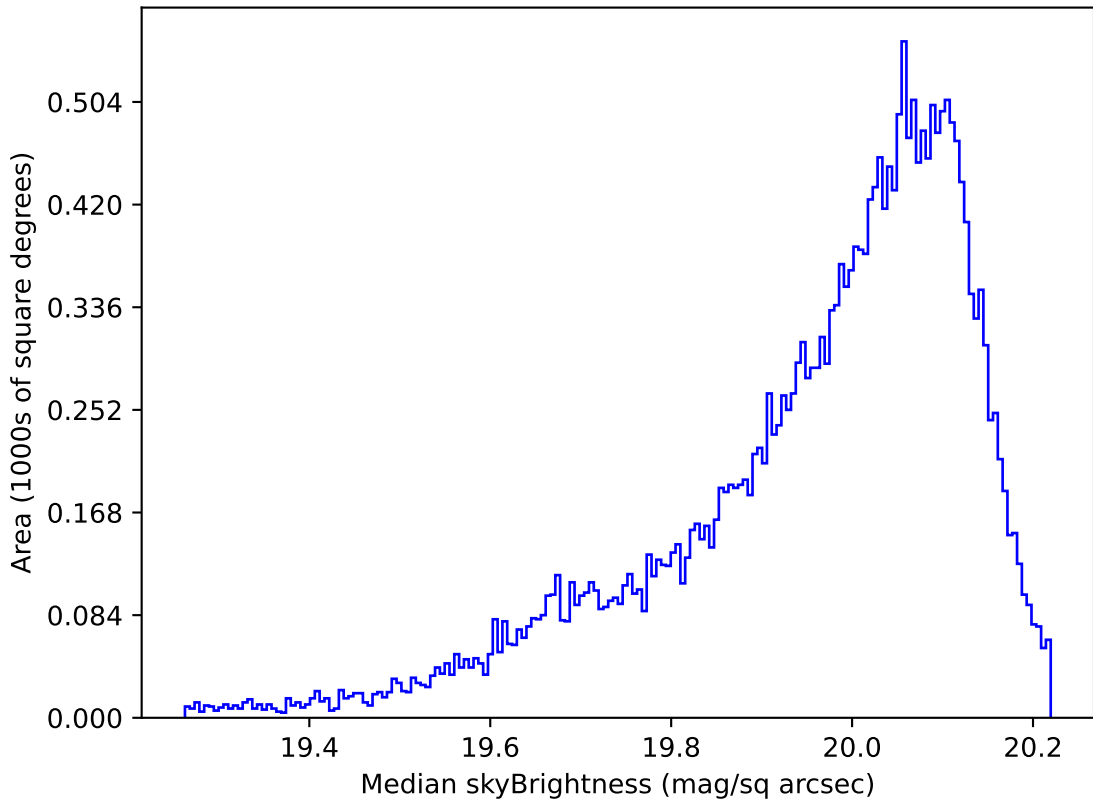
roll_pause_mjdp270_v3.4_10yrs All sky i band: Median skyBrightness
