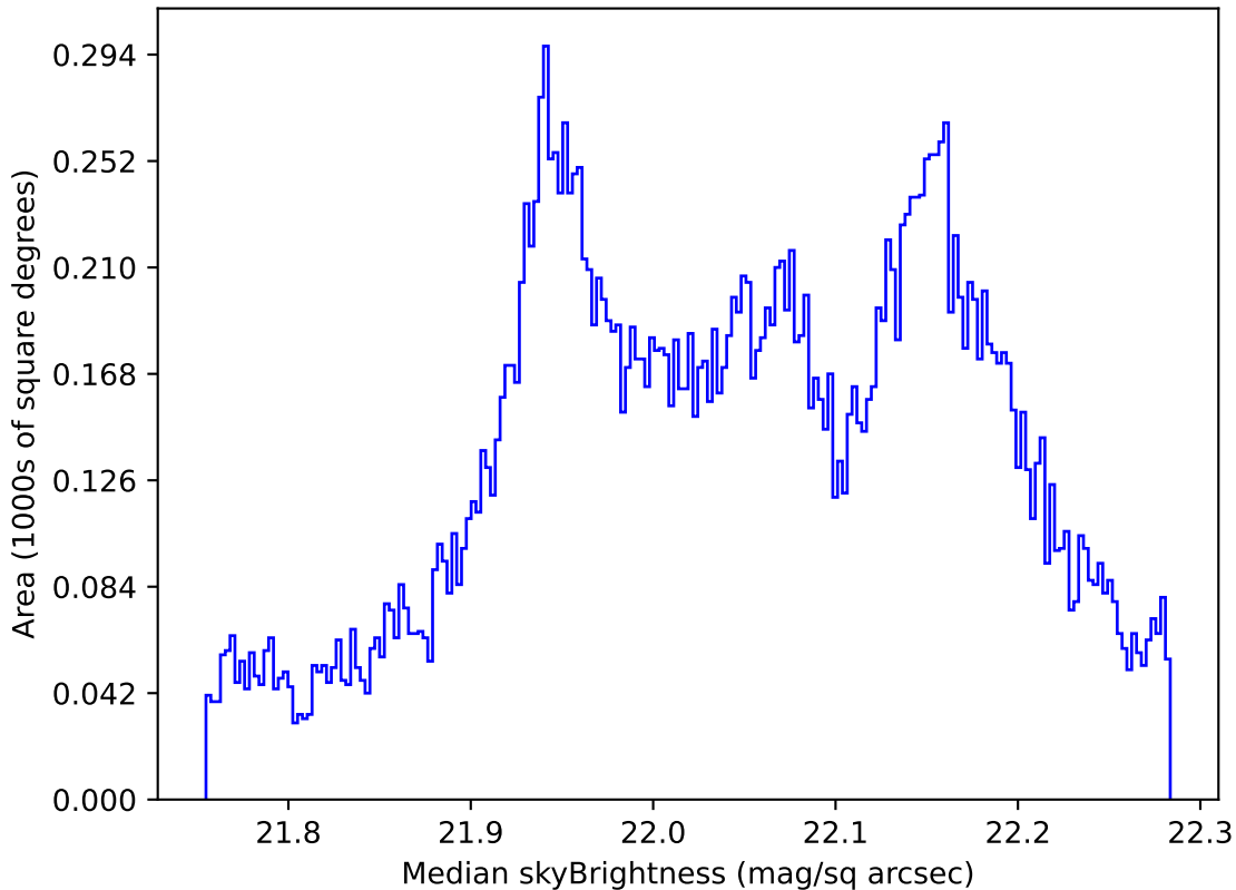
roll_pause_mjdp270_v3.4_10yrs All sky g band: Median skyBrightness
