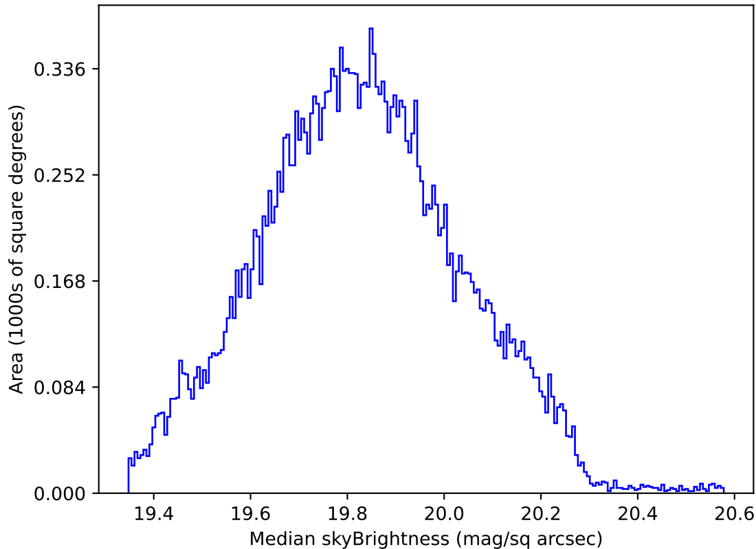
roll_pause_mjdp270_v3.4_10yrs All sky all bands: Median skyBrightness
