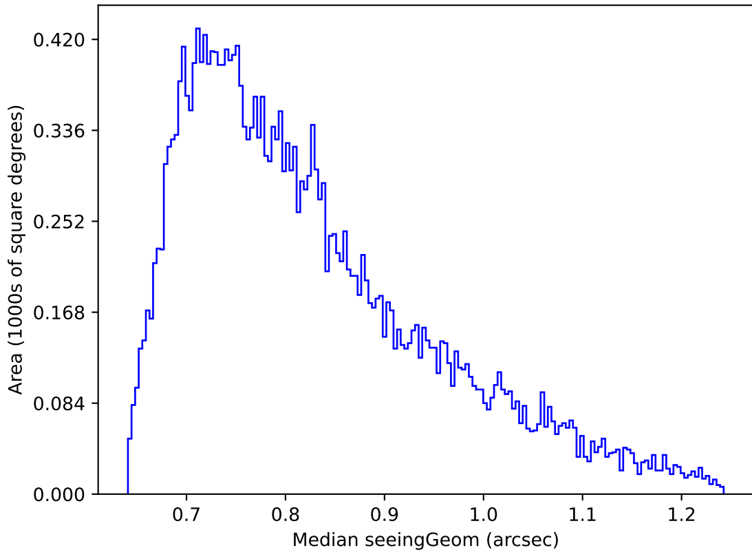
roll_pause_mjdp270_v3.4_10yrs Yr 1 r band: Median seeingGeom
