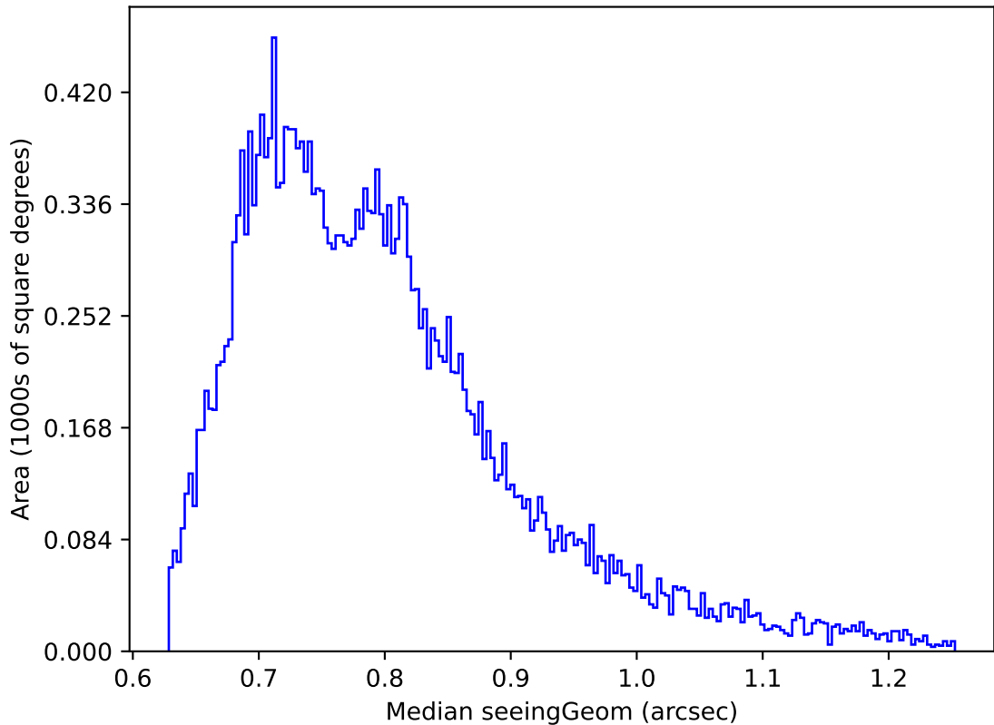
roll_pause_mjdp270_v3.4_10yrs Yr 1 i band: Median seeingGeom
