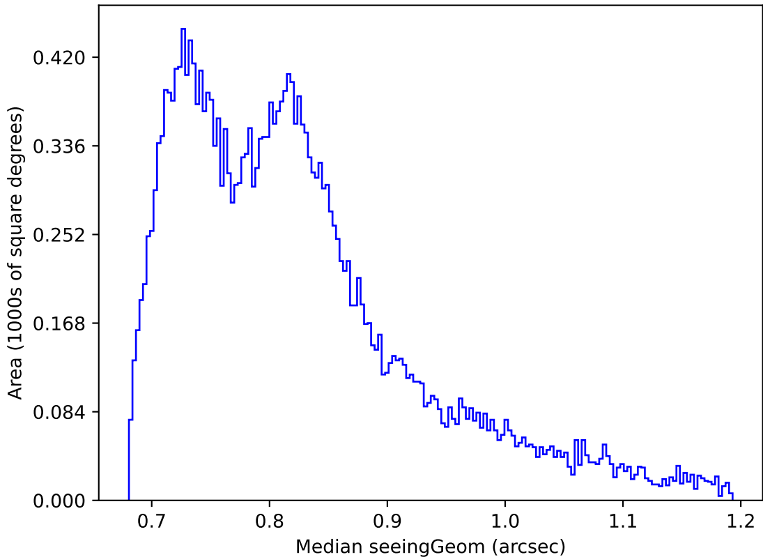
roll_pause_mjdp270_v3.4_10yrs Yr 1 all bands: Median seeingGeom
