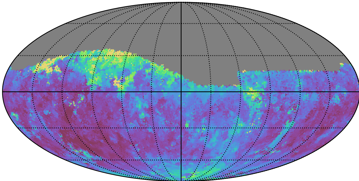
roll_pause_mjdp270_v3.4_10yrs Yr 1 z band: Median seeingEff
