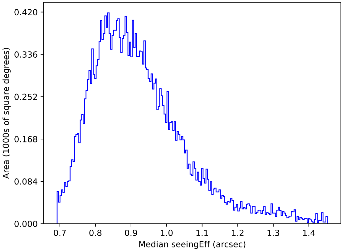
roll_pause_mjdp270_v3.4_10yrs Yr 1 z band: Median seeingEff
