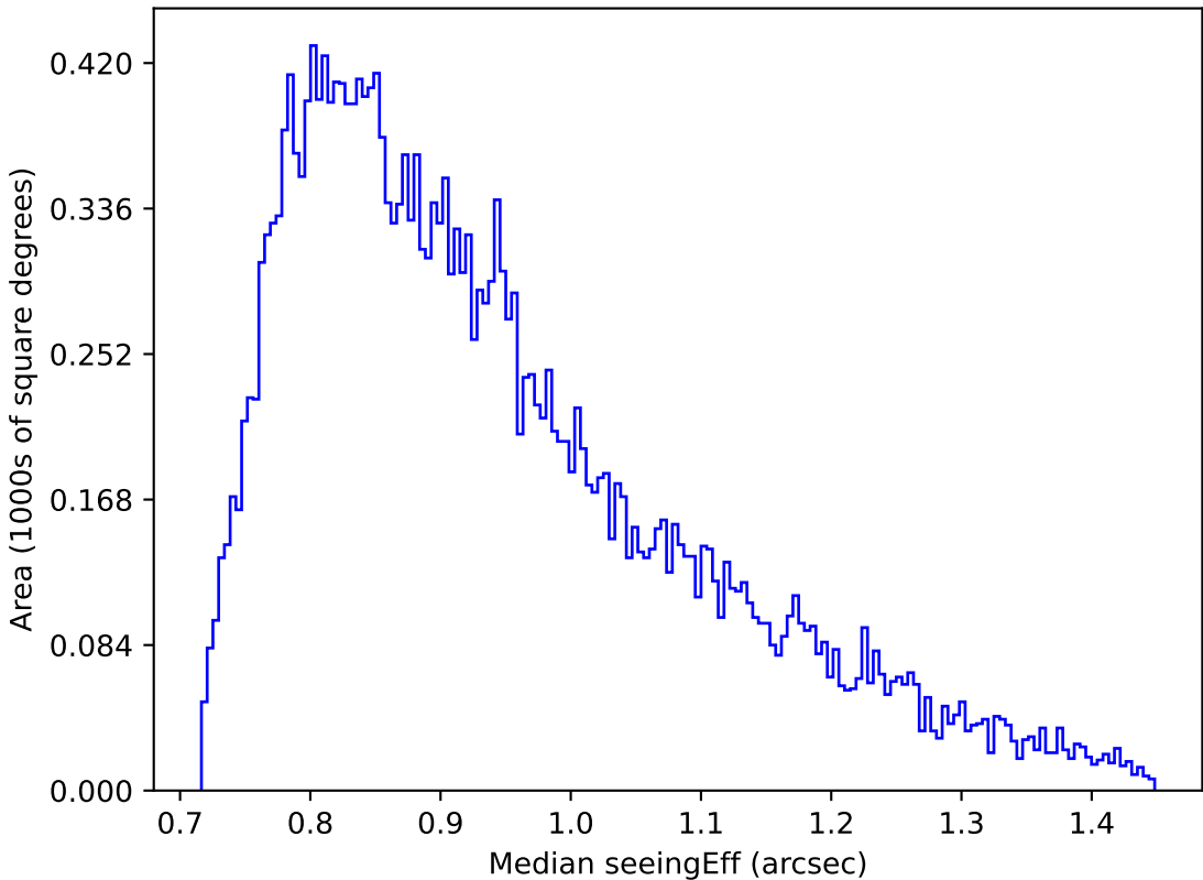
roll_pause_mjdp270_v3.4_10yrs Yr 1 r band: Median seeingEff
