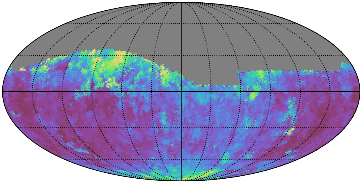
roll_pause_mjdp270_v3.4_10yrs Yr 1 i band: Median seeingEff
