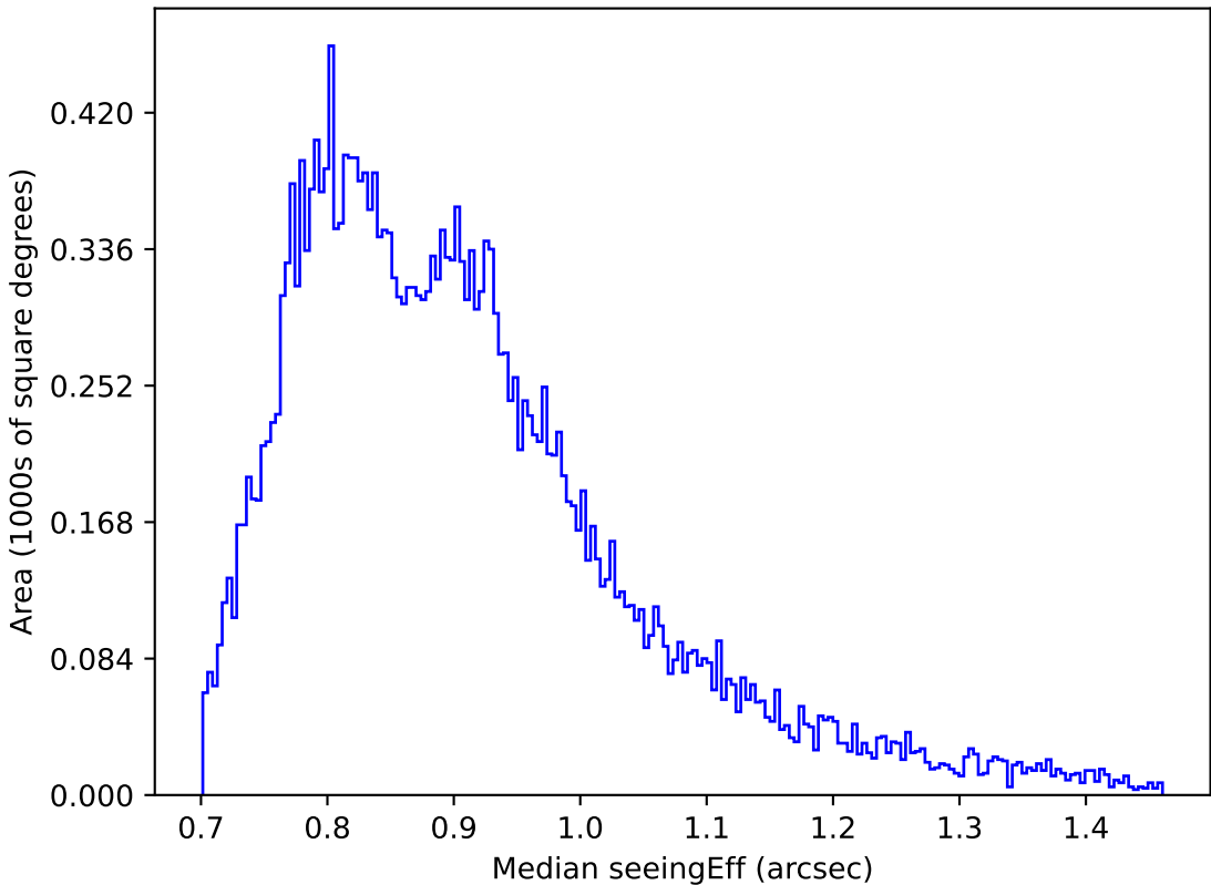
roll_pause_mjdp270_v3.4_10yrs Yr 1 i band: Median seeingEff
