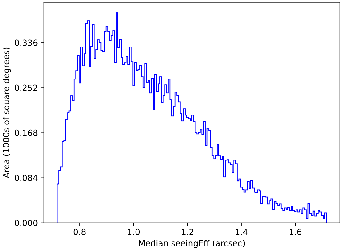
roll_pause_mjdp270_v3.4_10yrs Yr 1 g band: Median seeingEff
