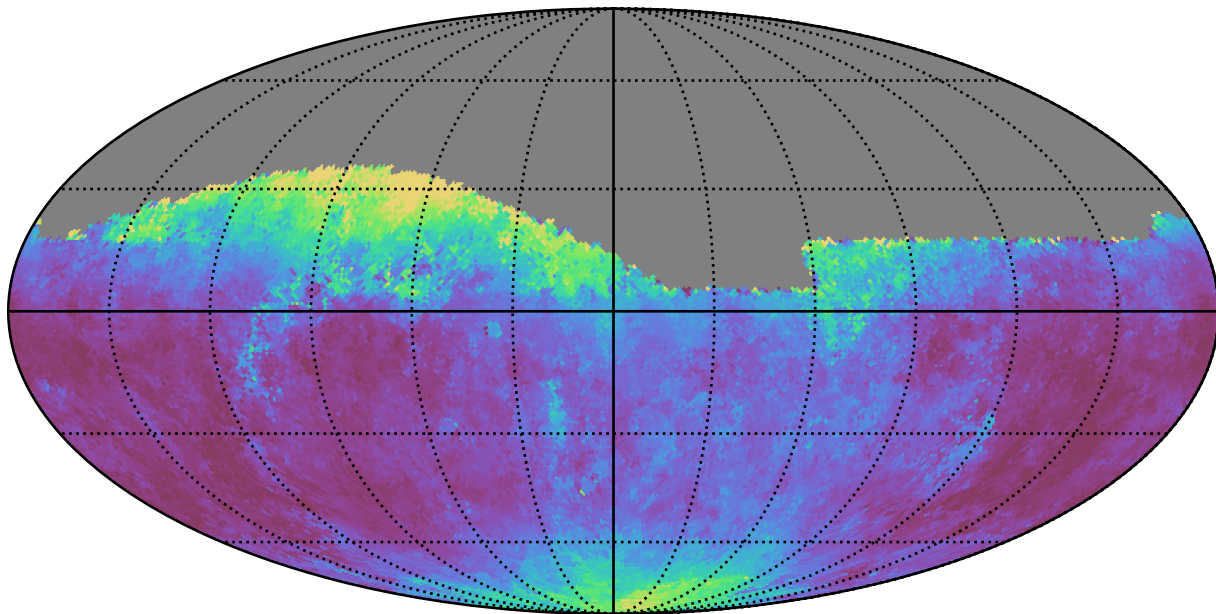
roll_pause_mjdp270_v3.4_10yrs Yr 1 all bands: Median seeingEff
