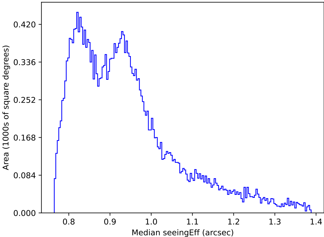
roll_pause_mjdp270_v3.4_10yrs Yr 1 all bands: Median seeingEff
