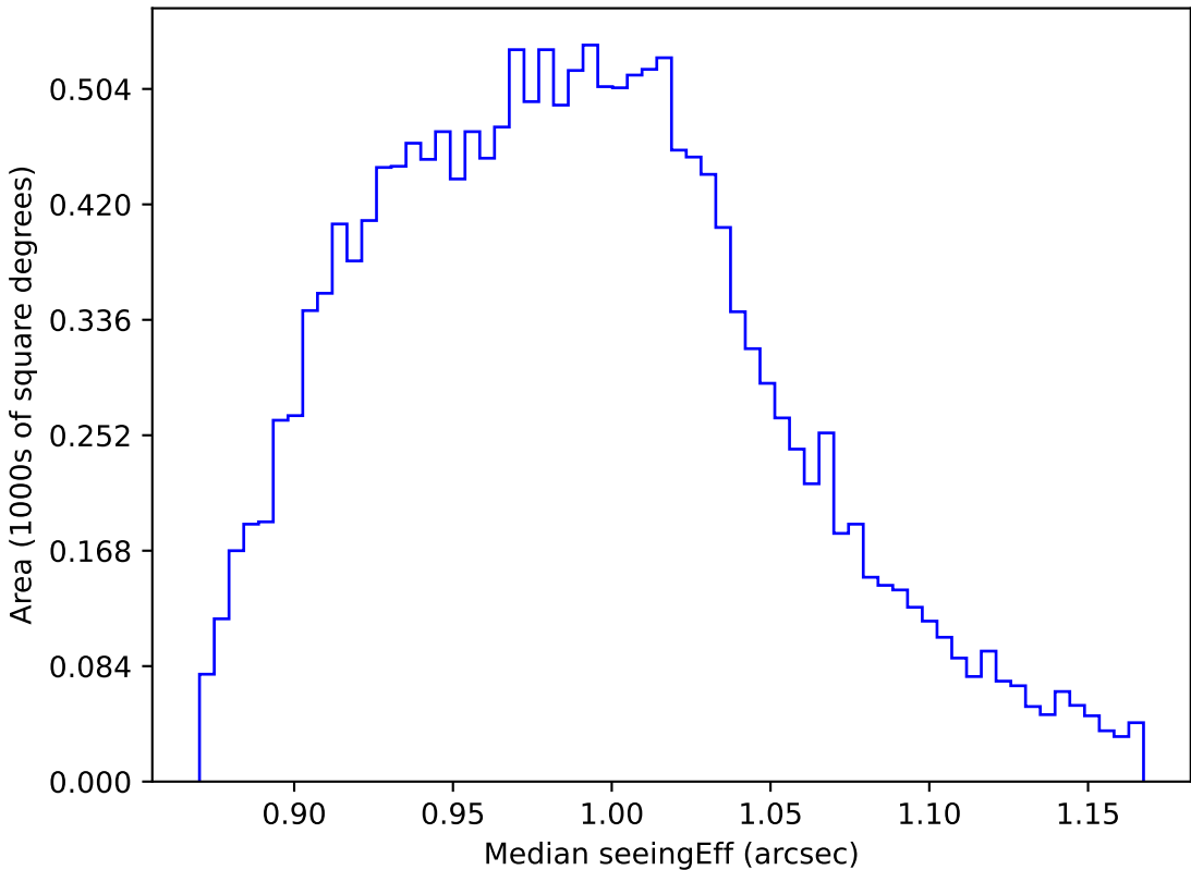
roll_pause_mjdp270_v3.4_10yrs WFD y band: Median seeingEff
