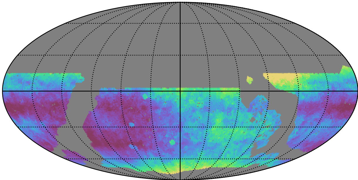
roll_pause_mjdp270_v3.4_10yrs WFD r band: Median seeingEff
