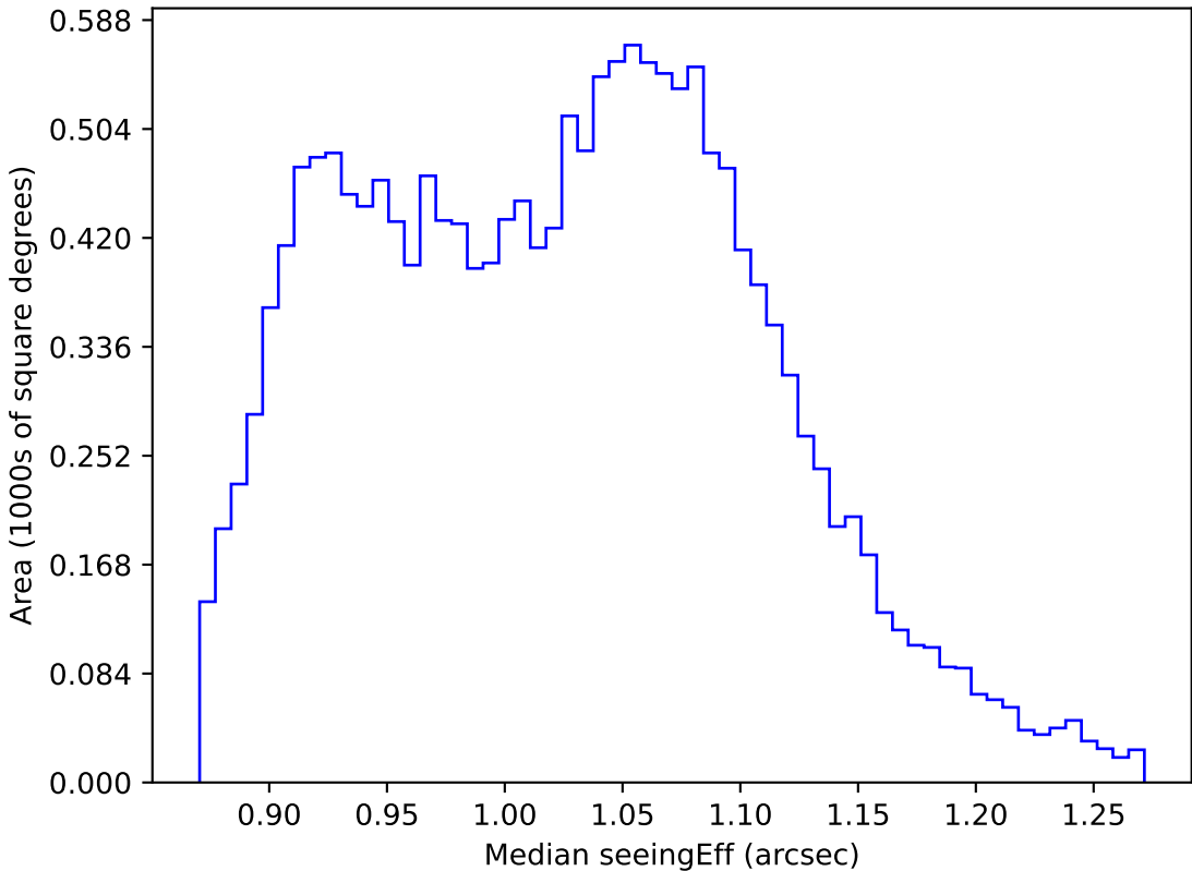
roll_pause_mjdp270_v3.4_10yrs WFD r band: Median seeingEff
