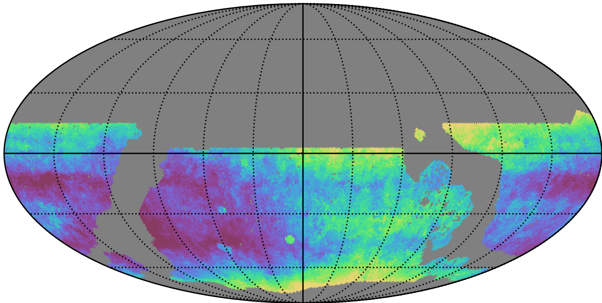
roll_pause_mjdp270_v3.4_10yrs WFD i band: Median seeingEff
