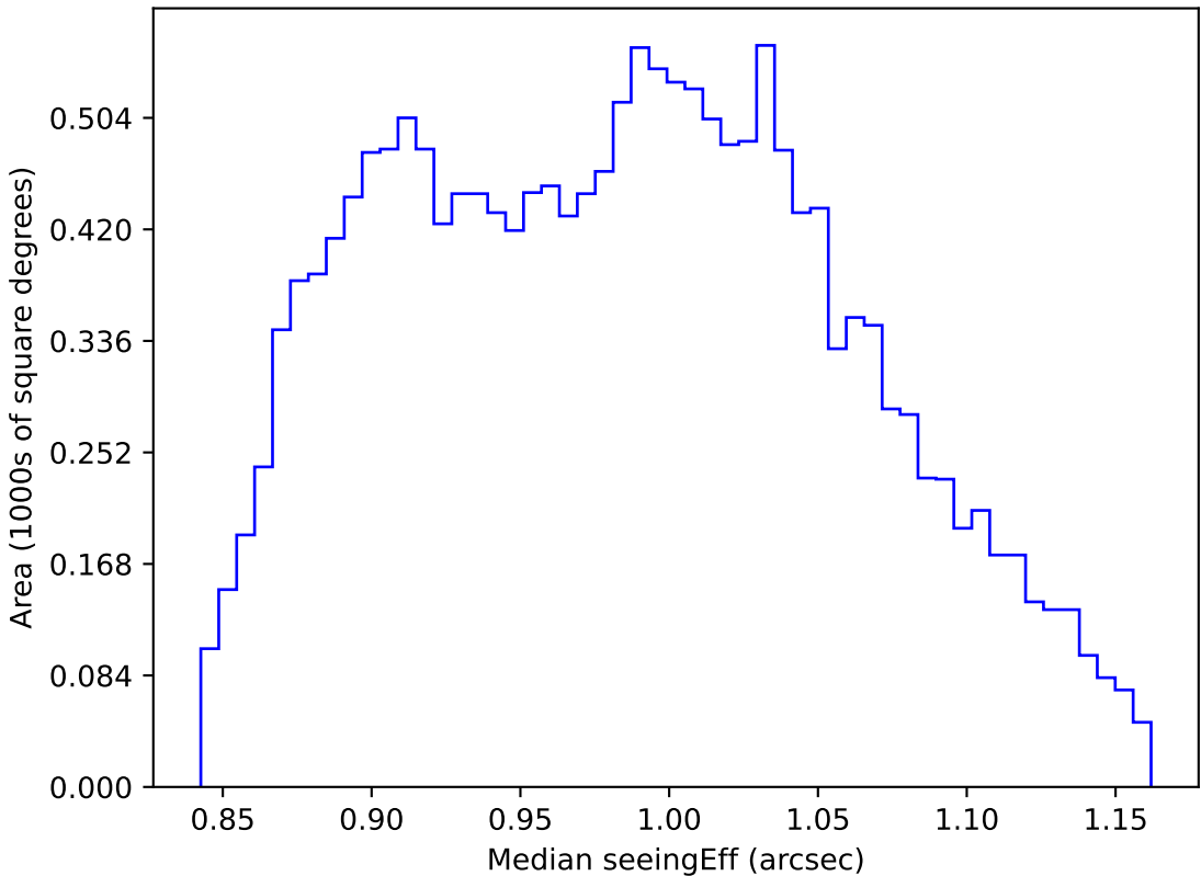
roll_pause_mjdp270_v3.4_10yrs WFD i band: Median seeingEff
