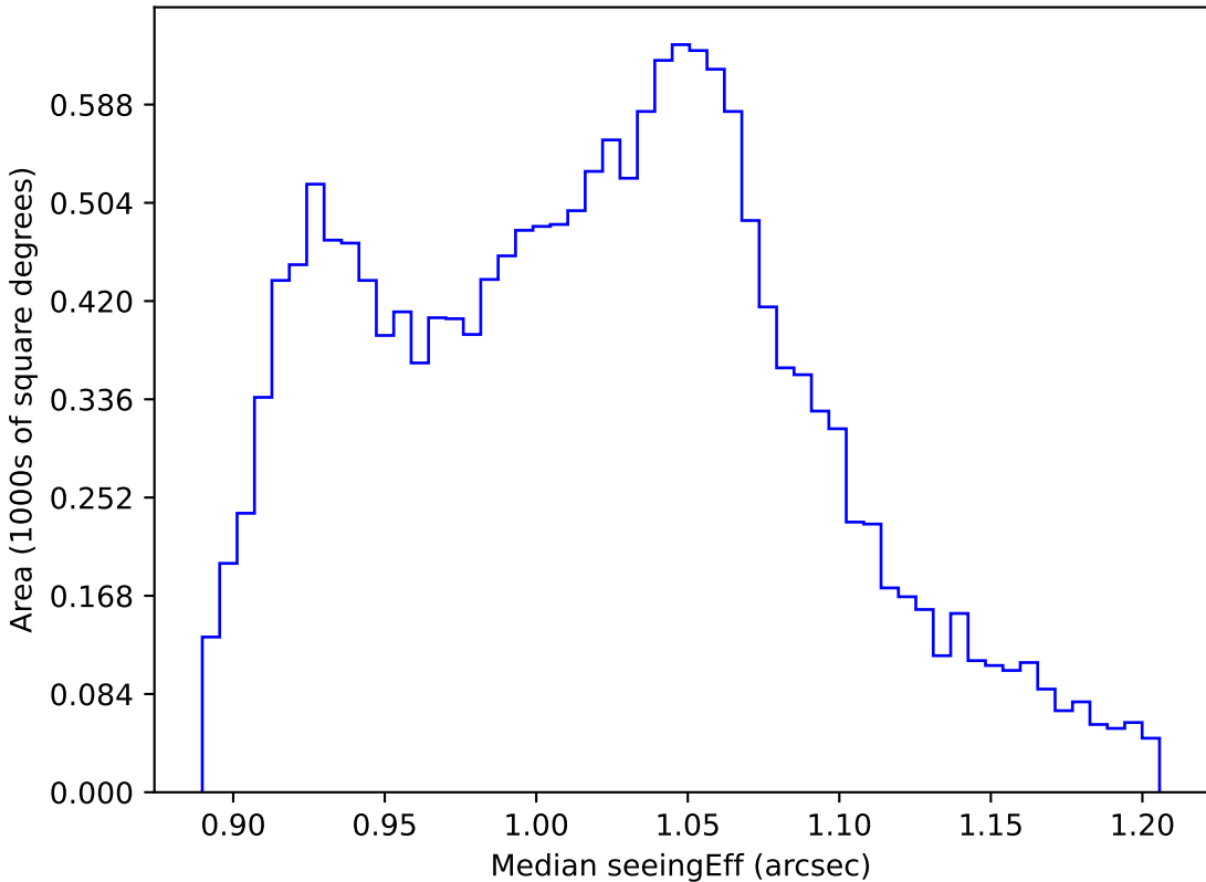
roll_pause_mjdp270_v3.4_10yrs WFD all bands: Median seeingEff
