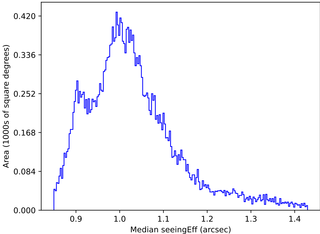
roll_pause_mjdp270_v3.4_10yrs All sky z band: Median seeingEff
