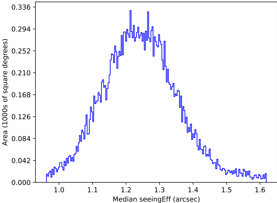
roll_pause_mjdp270_v3.4_10yrs All sky u band: Median seeingEff
