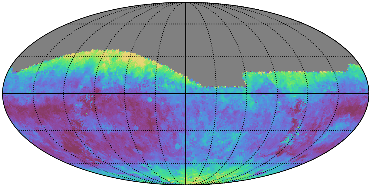
roll_pause_mjdp270_v3.4_10yrs All sky g band: Median seeingEff
