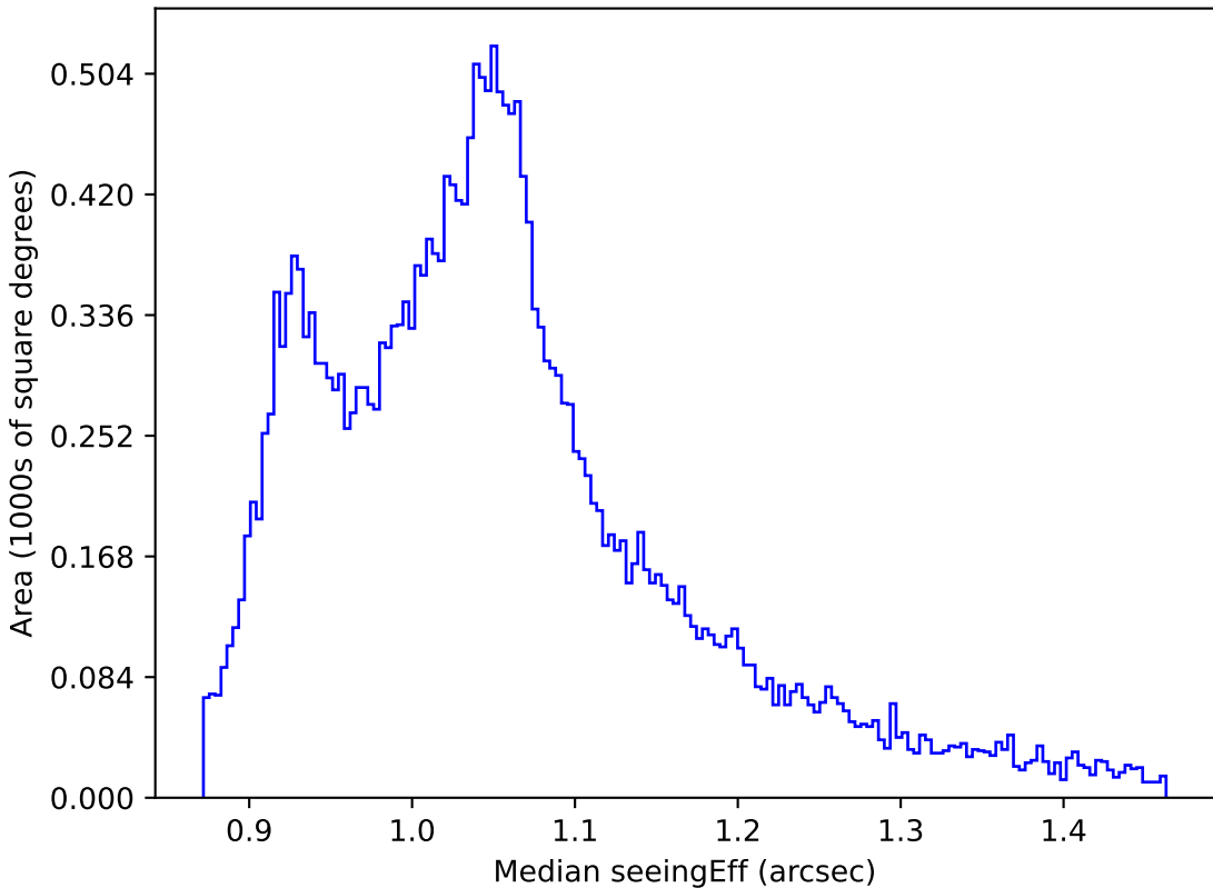
roll_pause_mjdp270_v3.4_10yrs All sky all bands: Median seeingEff
