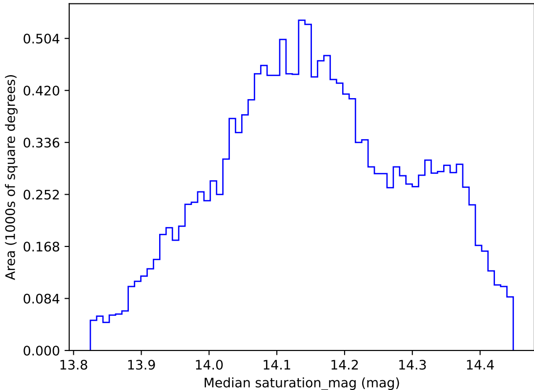
roll_pause_mjdp270_v3.4_10yrs WFD z band: Median saturation_mag
