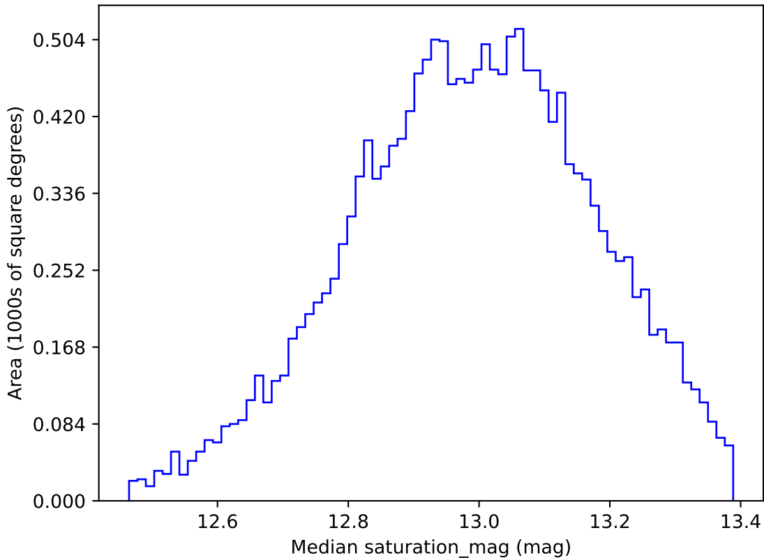
roll_pause_mjdp270_v3.4_10yrs WFD u band: Median saturation_mag
