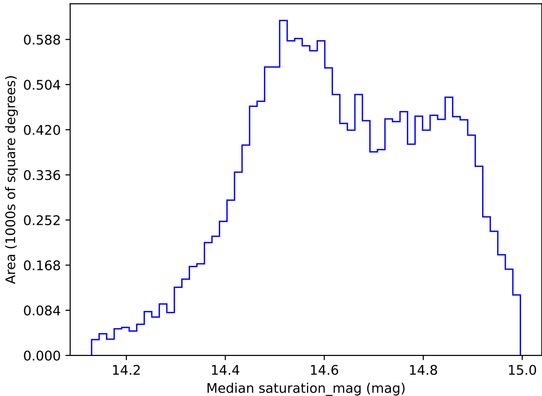
roll_pause_mjdp270_v3.4_10yrs WFD r band: Median saturation_mag
