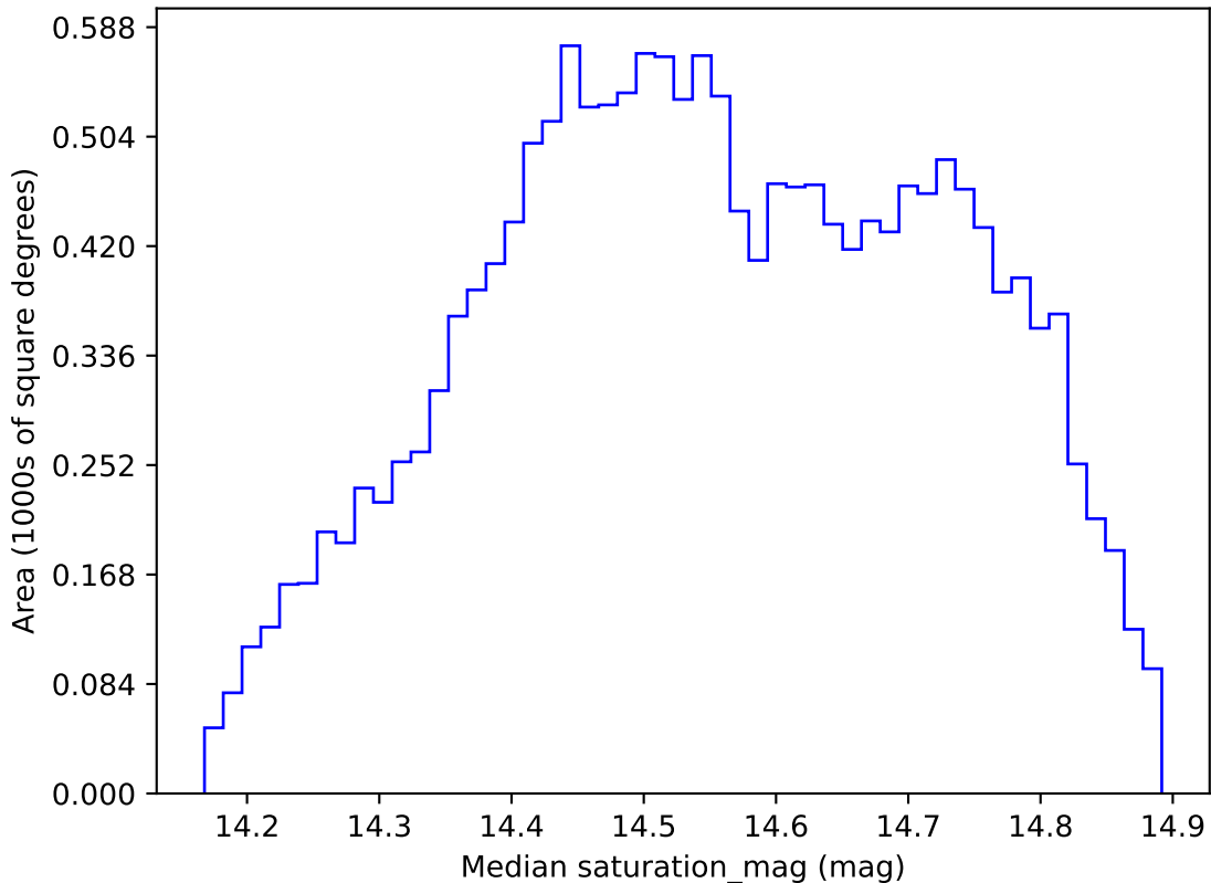
roll_pause_mjdp270_v3.4_10yrs WFD i band: Median saturation_mag
