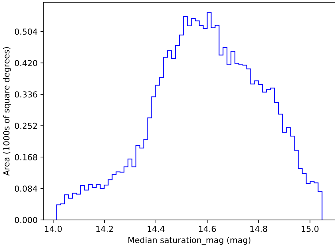
roll_pause_mjdp270_v3.4_10yrs WFD g band: Median saturation_mag
