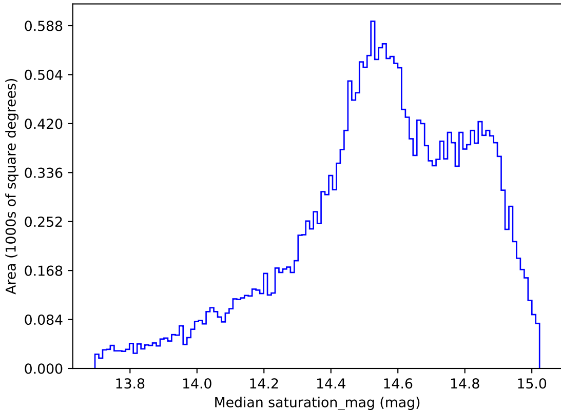
roll_pause_mjdp270_v3.4_10yrs All sky r band: Median saturation_mag
