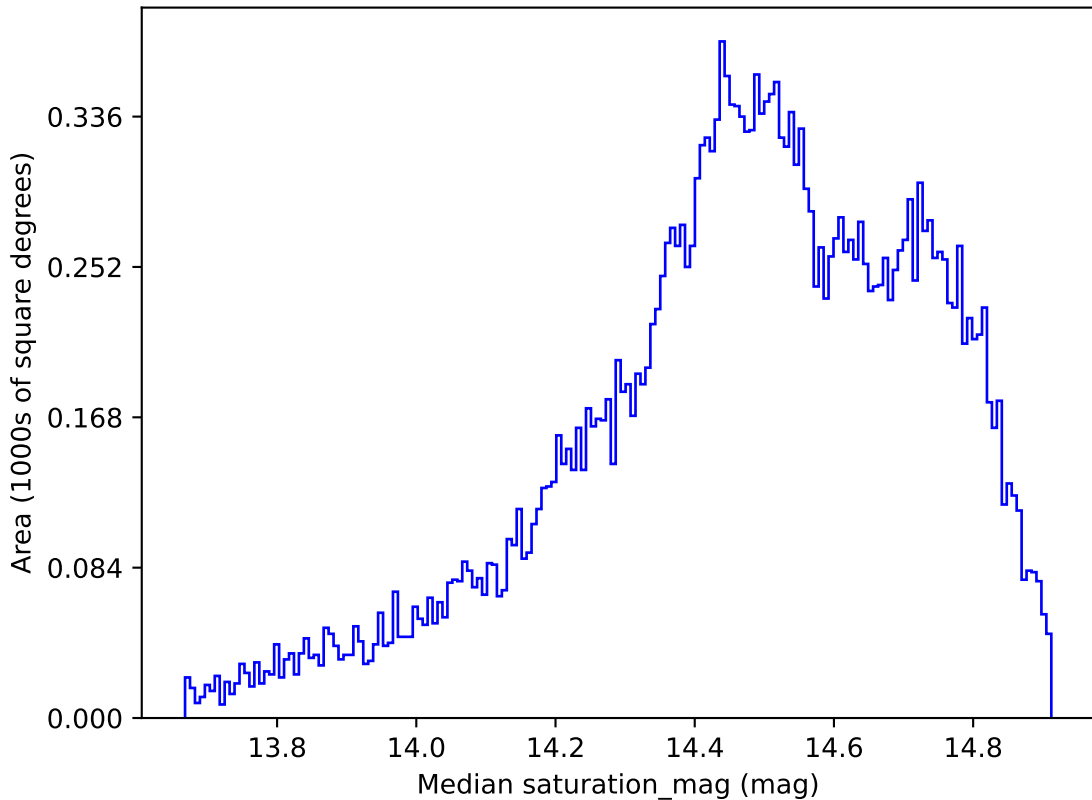
roll_pause_mjdp270_v3.4_10yrs All sky i band: Median saturation_mag
