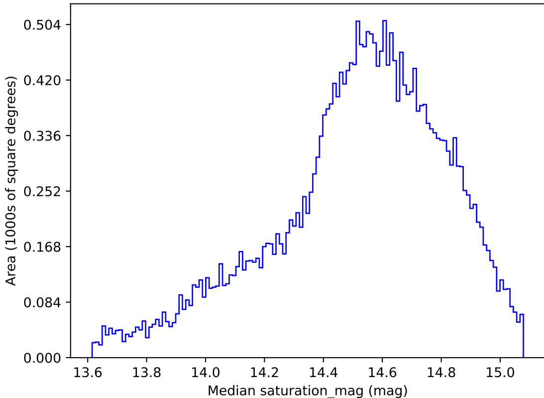
roll_pause_mjdp270_v3.4_10yrs All sky g band: Median saturation_mag
