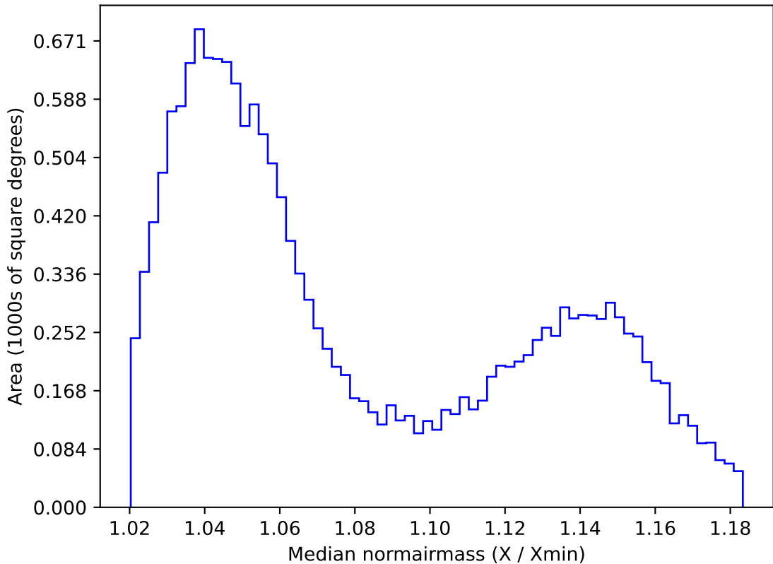
roll_pause_mjdp270_v3.4_10yrs WFD z band: Median normairmass
