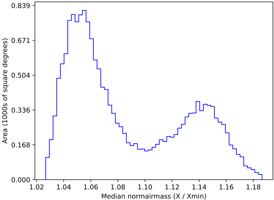
roll_pause_mjdp270_v3.4_10yrs WFD y band: Median normairmass
