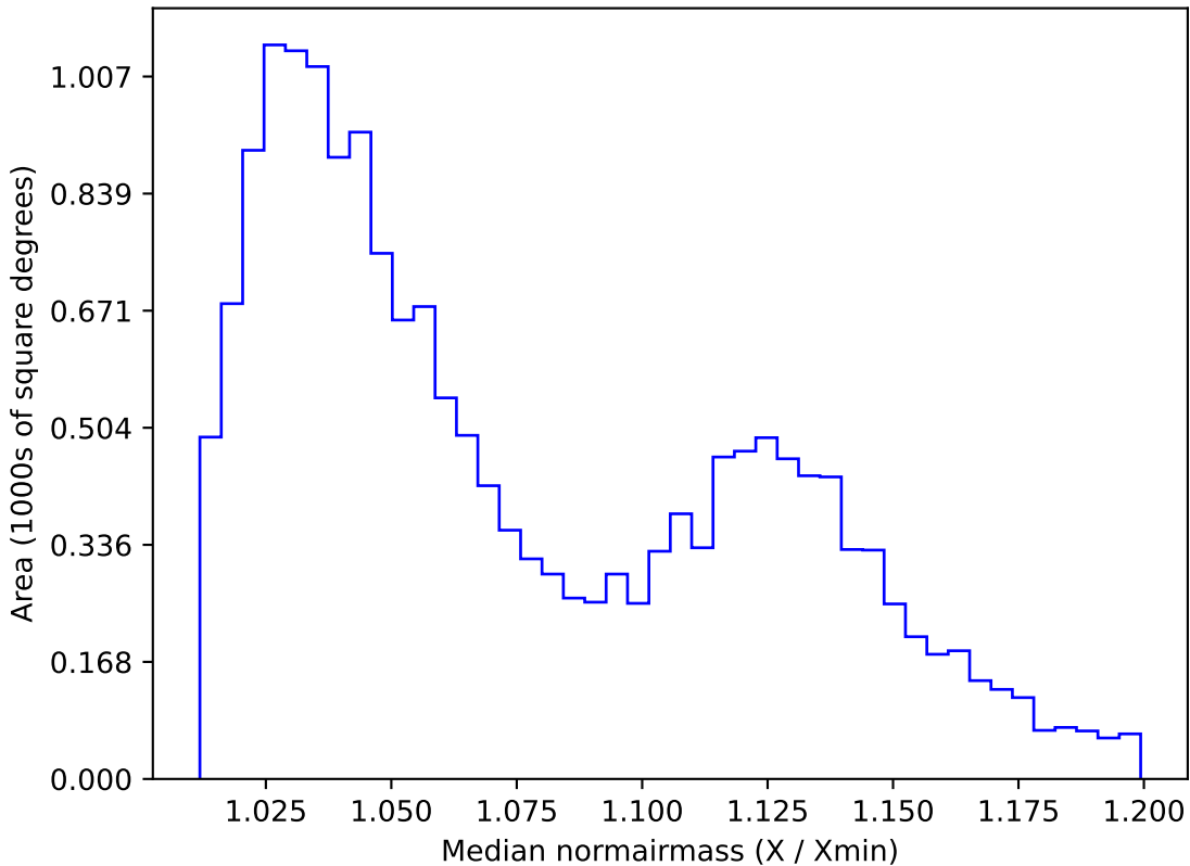
roll_pause_mjdp270_v3.4_10yrs WFD u band: Median normairmass
